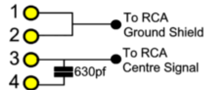
Male S-Video Plug
